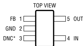
S5 PACKAGE 5-LEAD PLASTIC TSOT-23
